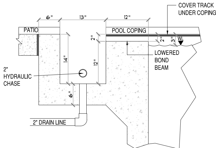
VAULT CROSS SECTION SCALE: 3/4" = 1'-0"
