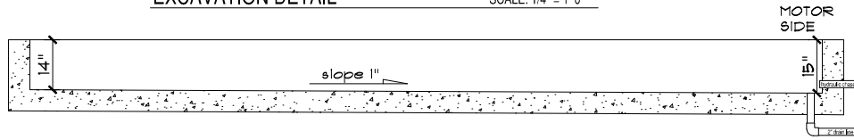
VAULT SECTION DETAIL SCALE: 1/4" = 1'-0"
