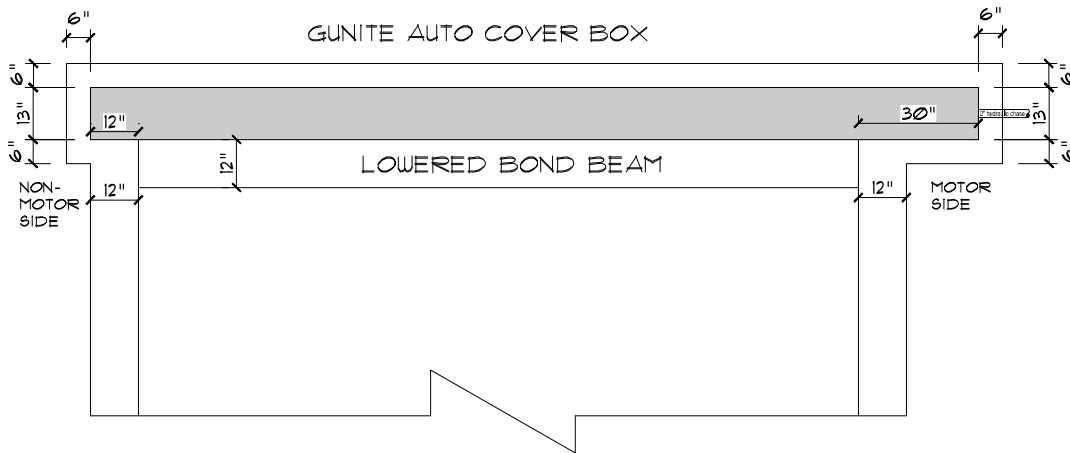
VAULT LAYOUT PLAN SCALE: 1/4" = 1'-0"
