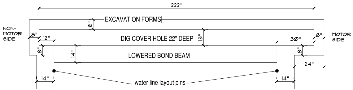
EXCAVATION DETAIL SCALE: 1/4" = 1'-0"
